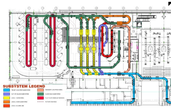
MF3 & MU3 Subsystem Overview
